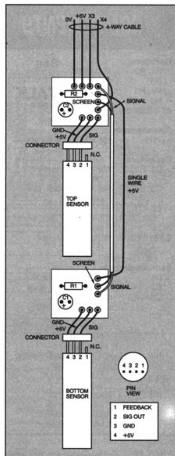
Fig.6. Sensor wiring details.
