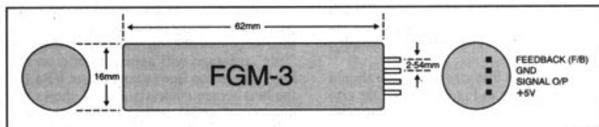
Fig.3. Details of the FGM-3 sensor module.
