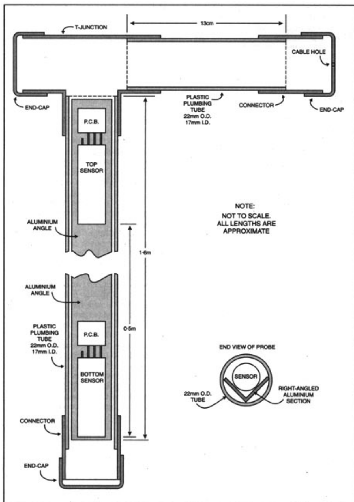
Fig.5. Probe assembly details.
